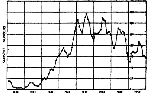
FIG. 6. THE TREND OF SUNSPOT ACTIVITY HAS BEEN DEFINITELY DOWNWARDS SINCE 1937. CURVE OF SUNSPOT NUMBERS SMOOTHED BY THREE MONTHS MOVING AVERAGES.
